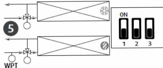
4 pipes with valve - Cooling and heating
