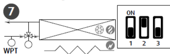
2 pipes with valve and electric heater Reversible/change over
