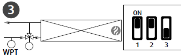
2 pipes with valve - Heating only
