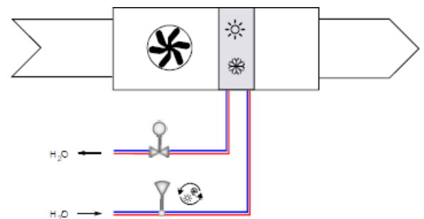
Figure 2-1 A two pipe system
