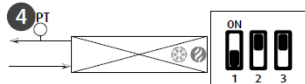
2 pipes without valve - Reversible/change over
