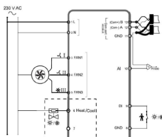
Figure 4-1 2-pipe wiring (standard)
