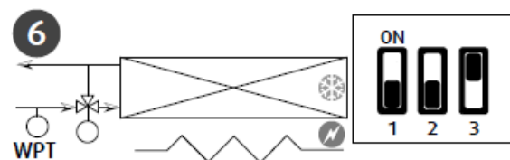
2 pipes with valve and electric heater Cooling/Heating
