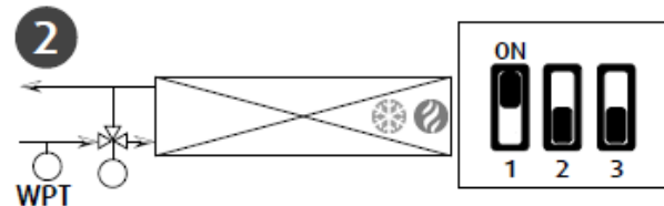
2 pipes with valve - Reversible/change over
