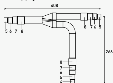
Suction piping
