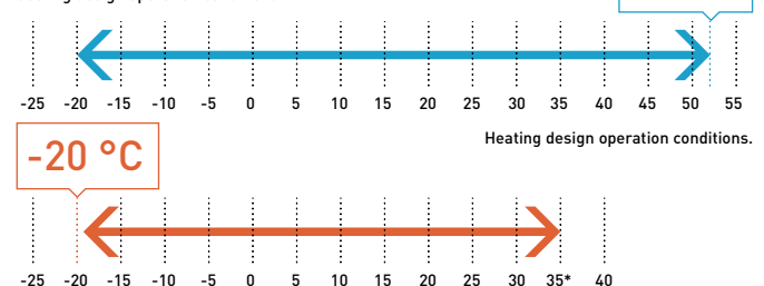
Cooling design operation conditions.
